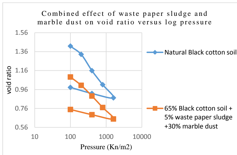
Fig. 4. Combined effects of waste paper sludge and marble dust on void ratio versus log pressure with loading and unloading for test pit 2
