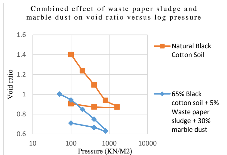
Fig. 3. Combined effects of waste paper sludge and marble dust on void ratio versus log pressure with loading and unloading for test pit 1
