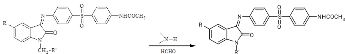
Scheme 2. Synthesis of N-Mannich bases
