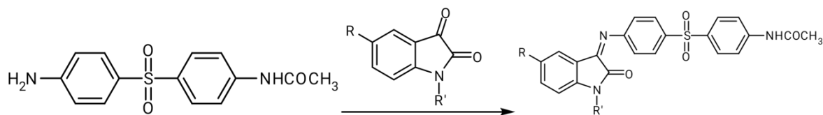
Scheme 1. Synthesis of Schiff's bases
