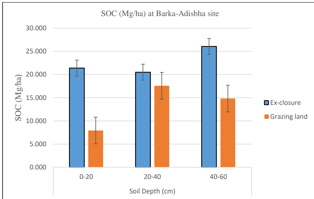
Fig. 2. Soil organic carbon variation with land use and soil depths
