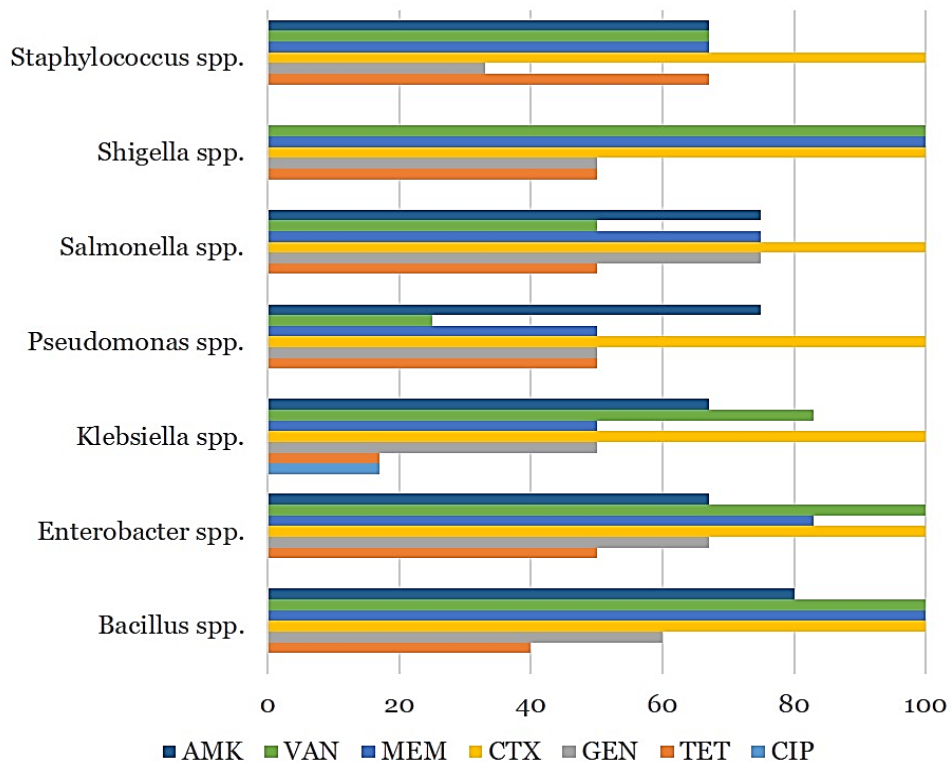
Fig. 4. Multiple antibiotics resistance pattern of bacterial isolates
