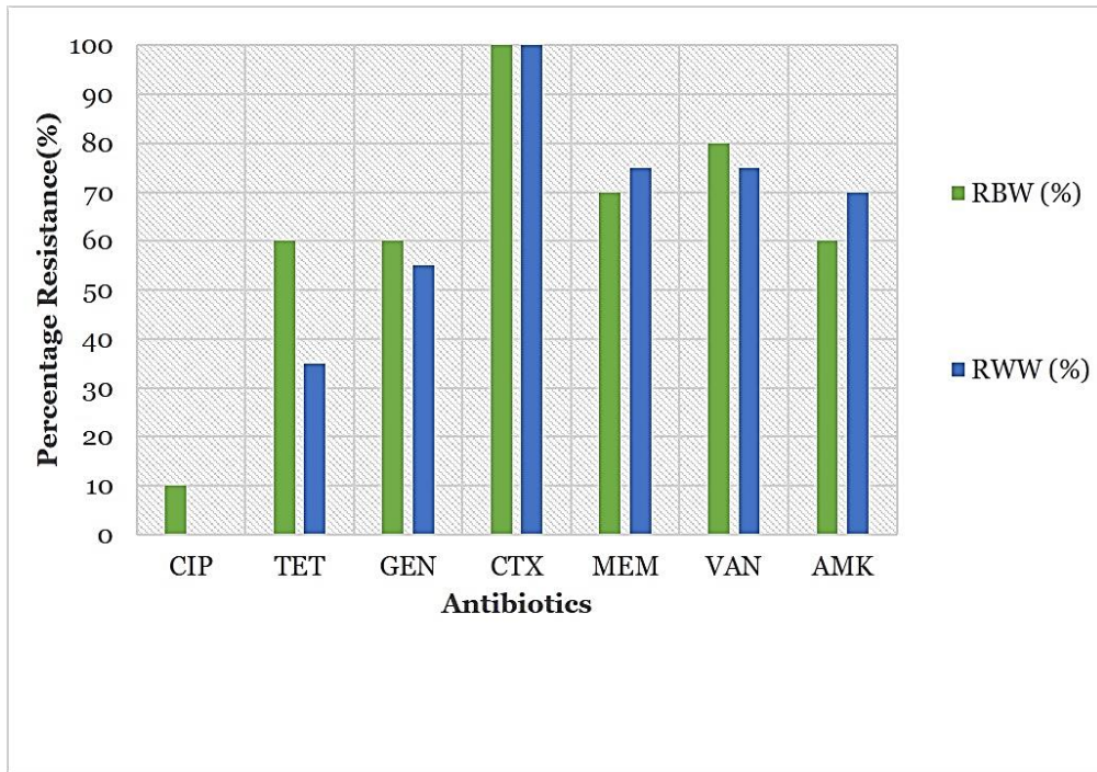
Fig. 3. Resistant pattern of bacterial isolates from well water and water from borehole storage tank
