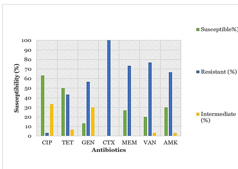
Fig. 2. Susceptibility pattern of bacteria isolated from water samples
