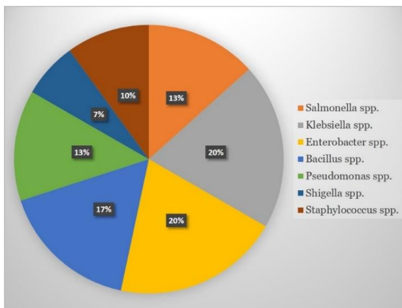
Fig. 1. Percentage incidence of bacterial isolate
