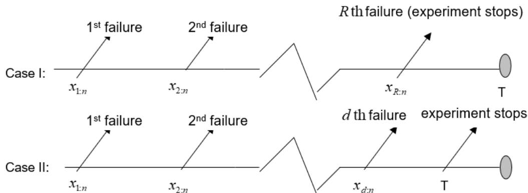
Fig. 1. Type-I hybrid censoring scheme
