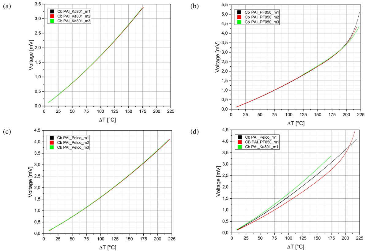
Figure 3. Recorded output for three consecutive measurements (m1–m3) over the temperature difference \Delta T (between junction and connections) for thermocouples consisting of: (a) Cb_PA I combined with Ka801; (b) carbon black in polyamide-imide combined with PF050; (c) carbon black in polyamide-imide combined with pelco. (d) Comparison of the characteristics of the three commercial thermocouples.
