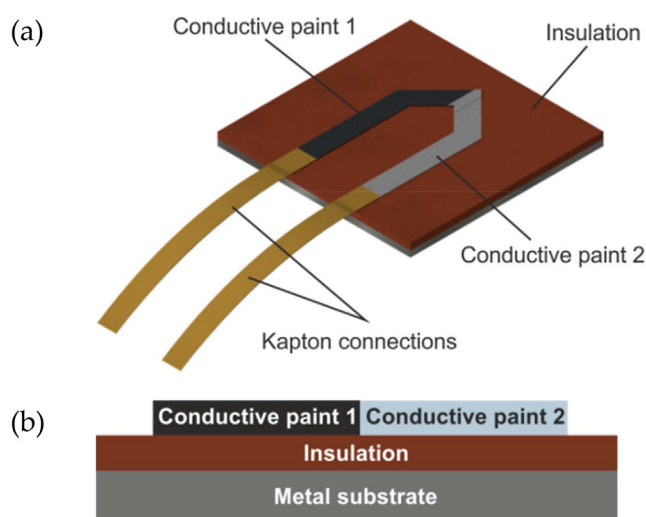
Figure 1. (a) Schematic depiction of the thermocouple consisting of the conductive paths on the insulated metal substrate and the connection strips, coated with the according conductive paint. (b) Layer architecture of the thermocouple.
