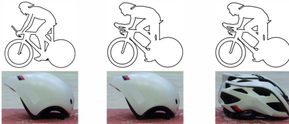
Figure 3. Riding configurations and helmets used. Upright position with aerodynamic helmet (left). Time trial position with aerodynamic helmet (middle). Time trial position with conventional road helmet (right).
