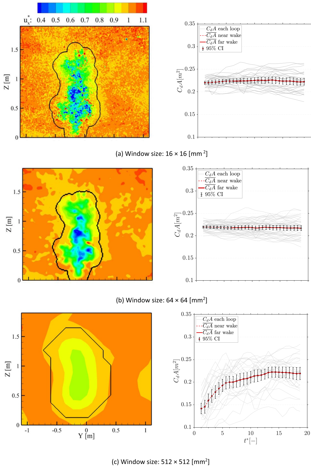
Figure 9. Dimensionless instantaneous streamwise velocity ( u_x^* ) at t^* = 1 (left) and streamwise C_dA evolution in the wake (right). Data from the individual test in time trial position with aerodynamic helmet. The black lines represent the wake contours used for the drag analysis. (a) Window size: 16 \times 16 [mm 2 ]. (b) Window size: 64 \times 64 [mm 2 ]. (c) Window size: 512 \times 512 [mm 2 ].
