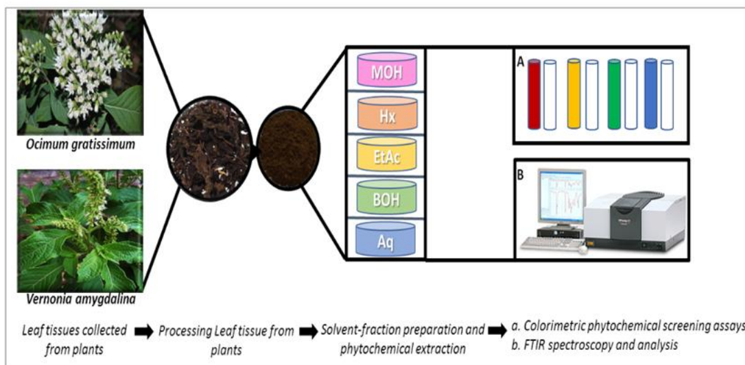
Fig. 2. Diagrammatical illustration of an experimental methodology for this study. The two medicinal plants ( Vernonia amygdalina and Ocimum gratissimum ) were used as a model for this study. Their leaves were harvested, dried, processed, and differentially fractionated in various organic solvents to determine differences in phytochemical expression profiles via both phytochemical screening assays and FTIR spectroscopy methods. Organic solvents: MOH: methanol; Hx: hexane; EtAc: ethyl acetate; BOH: butanol; Aq: aqueous distilled water
