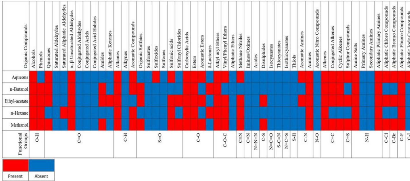
Fig. 7. Secondary metabolite or phytochemical expression profile of different solvent-fractions of Vernonia amygdalina leaf tissue extract. Heatmap represents the relative expression profile of secondary metabolites phytochemical compounds expressed in leaf tissue of different organic solvent-fractions analyzed with FTIR spectroscopy based on functional group determination
