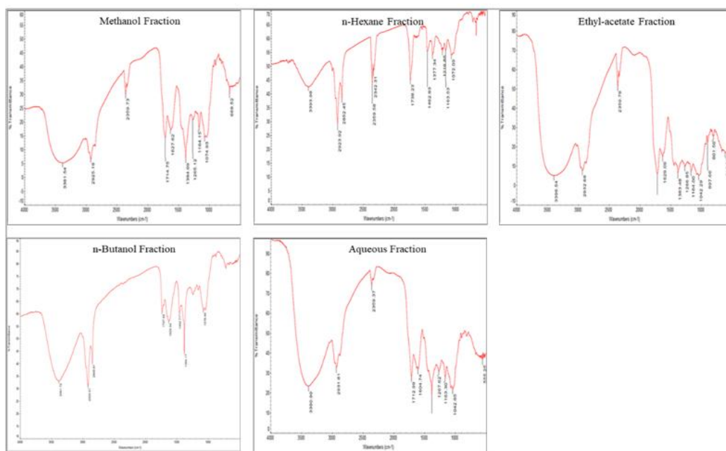
Fig. 5. FTIR spectra of methanolic, n-hexane, ethyl-acetate, n-butanol, and aqueous solvent-fractions of Vernonia amygdalina leaf tissue extracts
