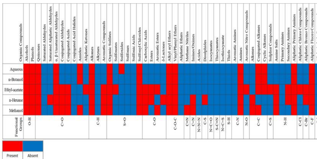
Fig. 6. Secondary metabolite/phytochemical expression profile of different solvent-fractions of Ocimum gratissimum leaf tissue extract. heatmap represents the relative expression profile of secondary metabolites/ phytochemical compounds expressed in leaf tissue of different organic solvent-fractions analyzed with FTIR spectroscopy based on functional group determination
