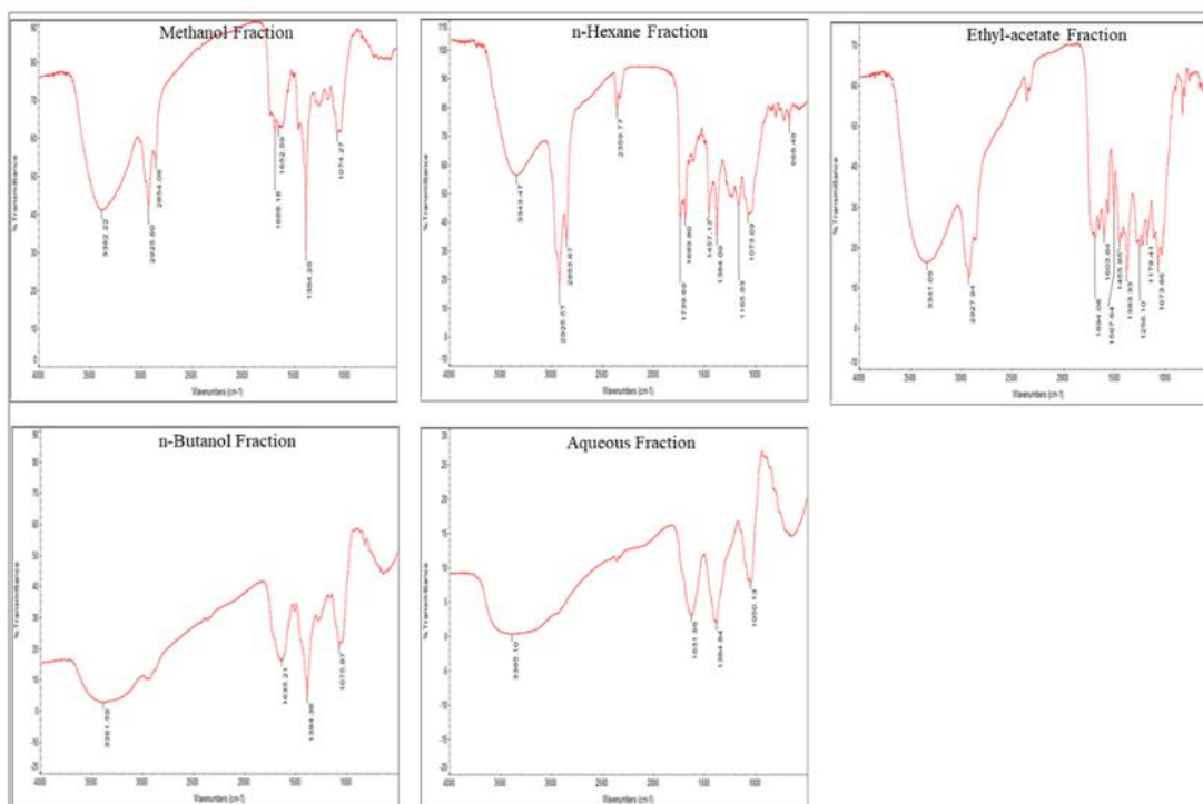
Fig. 4. FTIR spectra of methanolic, n-hexane, ethyl-acetate, n-butanol, and aqueous solvent-fractions of Ocimum gratissimum leaf extracts
