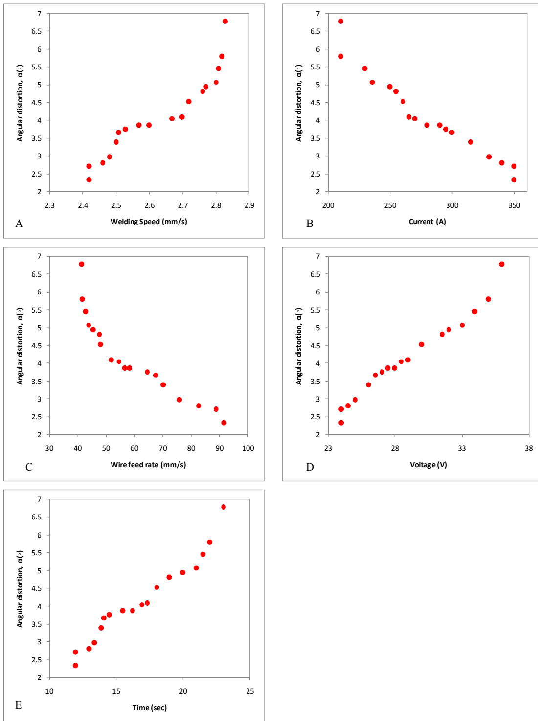
Fig. 2. Effect of process parameters on angular distortion
