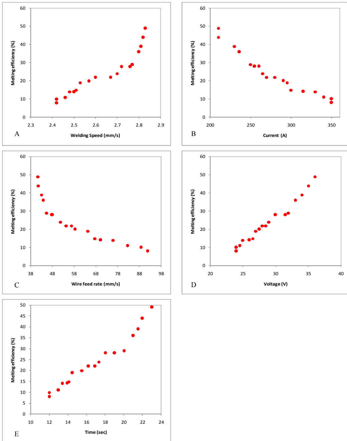
Fig. 6. Effect of process parameters on melting efficiency
