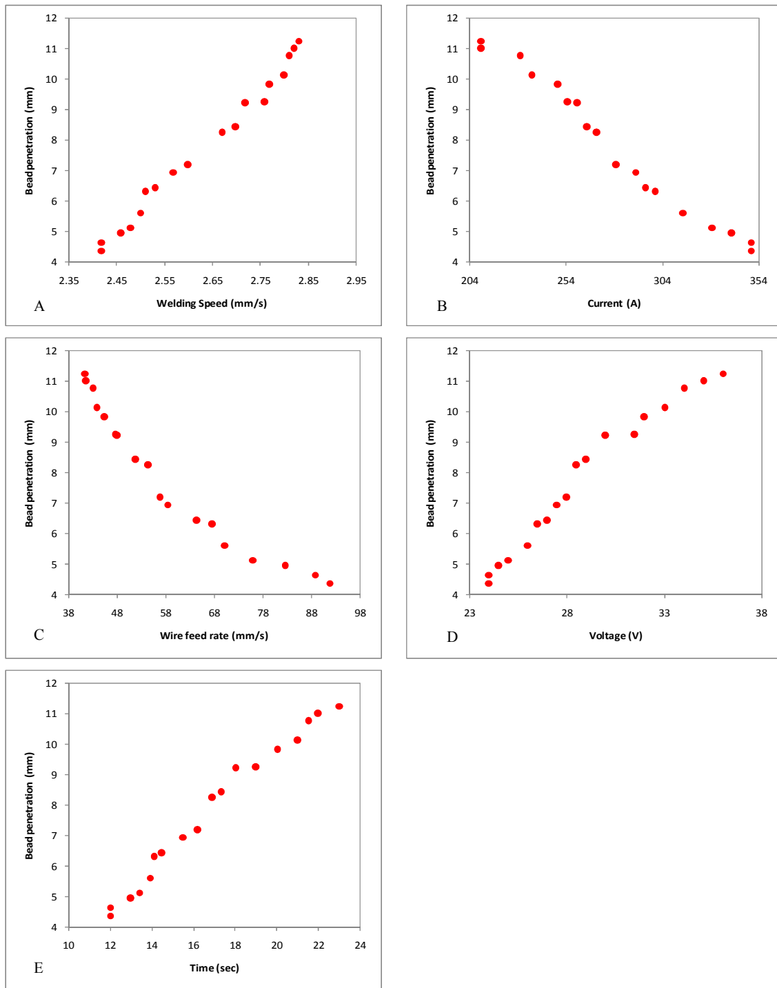
Fig. 4. Effect of process parameters on bead penetration
