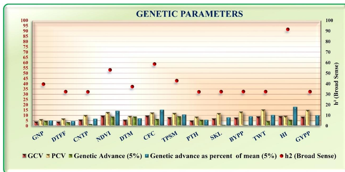
Fig. 1. Graphical representation of genetic parameters of variation (GCV, PCV, genetic advance (5%), genetic advance as percent of mean (5%), h 2 b for 13 traits among 50 bread wheat accessions
