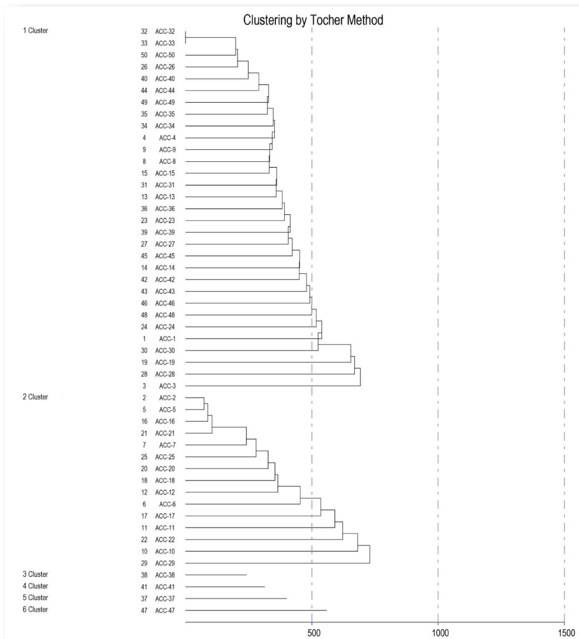
Fig. 2. Dendrogram of 50 bread wheat accessions for 13 traits
