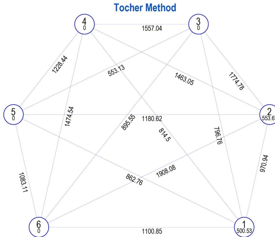
Fig. 3. Cluster diagram of 50 bread wheat accessions using Tocher method
