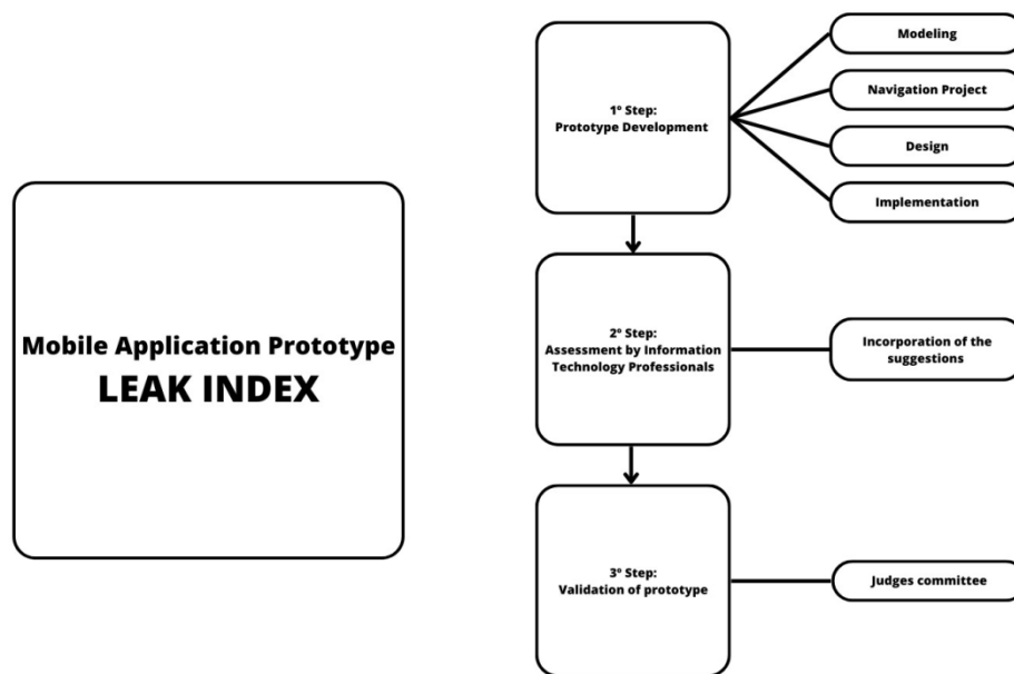
Fig. 1. Flowchart of the study steps. Belo Horizonte, Minas Gerais, Brazil, 2022
